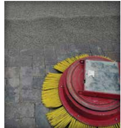
Figure 27 and 28. Mechanical equipment accelerated installation of a parking lot in Illinois and a street in Oregon.
